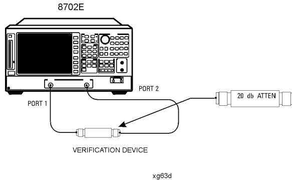
Figure 3-3. Connections for the 20 dB Verification Device
