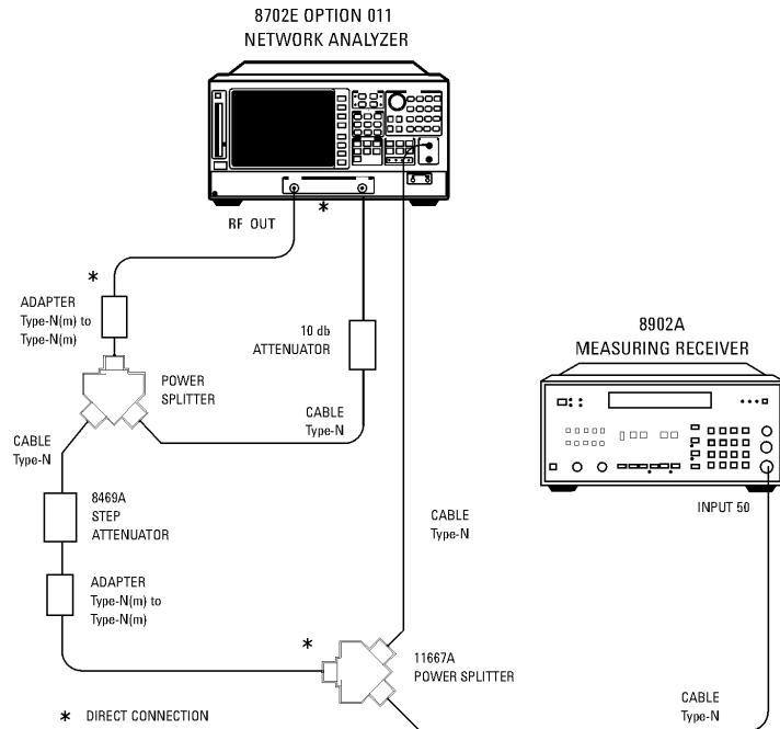
Figure 6-24. Channel R Magnitude Dynamic Accuracy Test Setup
