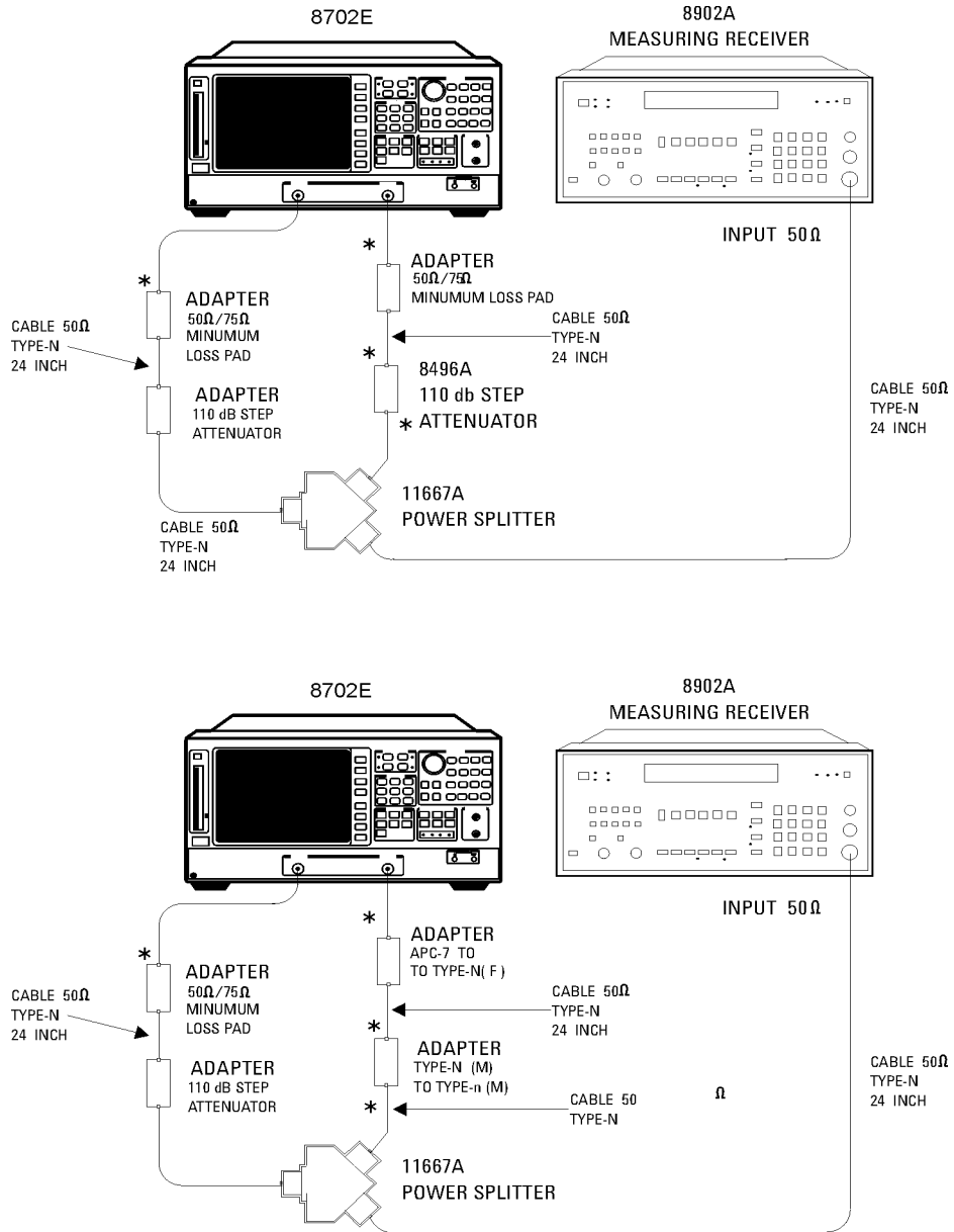
Figure 4-31. Test Port 2 Dynamic Accuracy Test Setup
