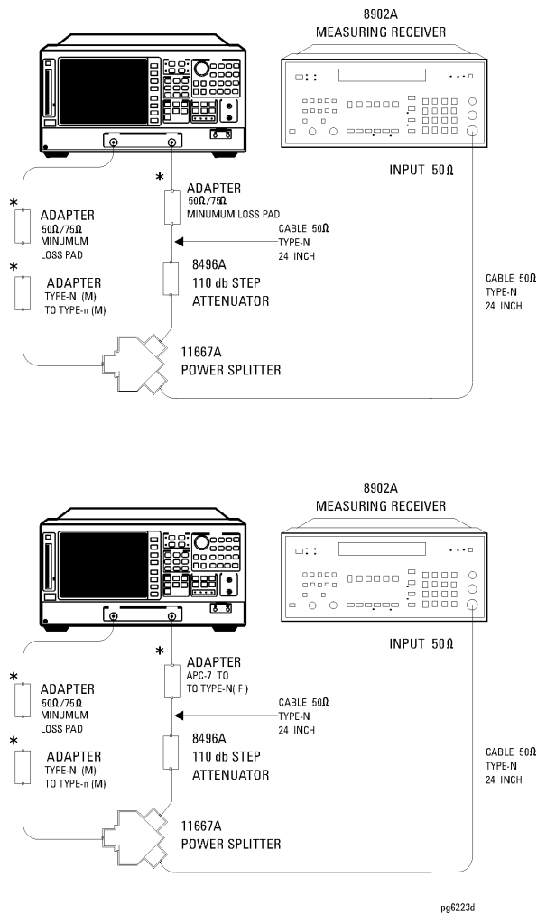
Figure 4-32. Test Port 1 Magnitude Dynamic Accuracy Test Setup
