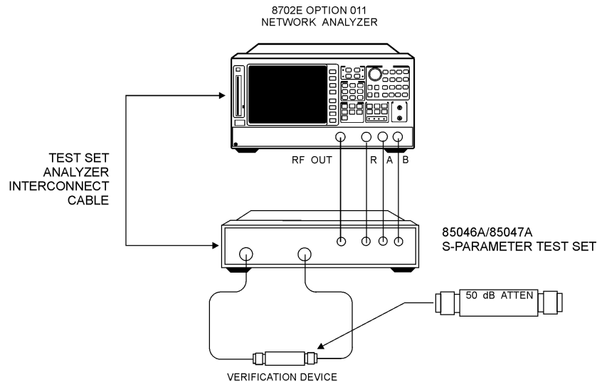
Figure 5-5. Connections for the 50 dB Verification Device
