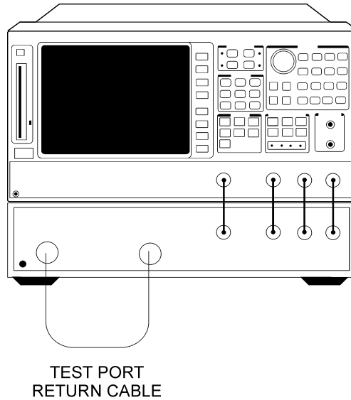
Figure 1-19. Transmission Mode Connections
