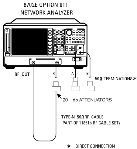
Figure 6-7. Receiver Channel Noise Floor Level Test Setup
