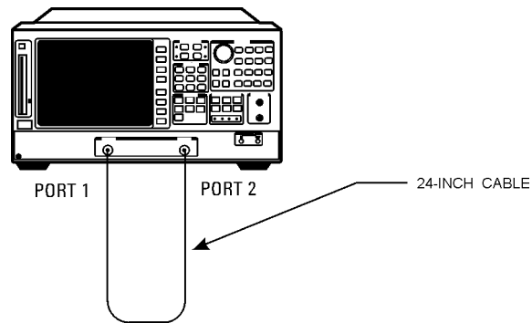
Figure 4-11. Test Port 2 Input Frequency Response Test Setup
