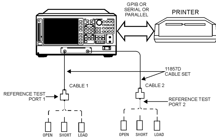
Figure 3-1. System Verification Test Setup
