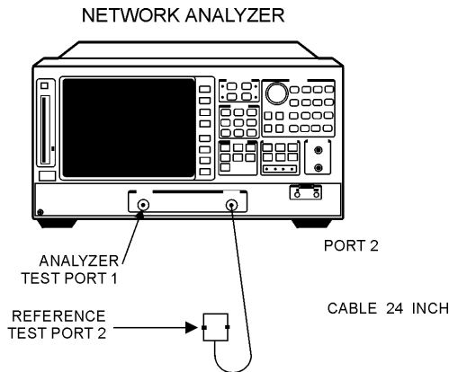
Figure 4-20. First Full 2-Port Calibration Test Setup
