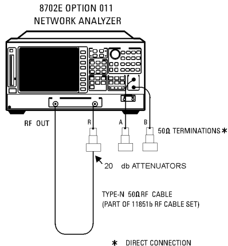
Figure 6-8. Receiver Channel Noise Floor Level Test Setup
