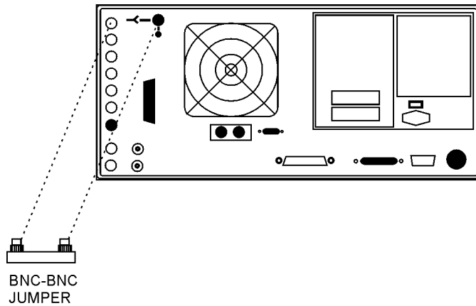
Figure 1-2. Jumper Cable Connection
