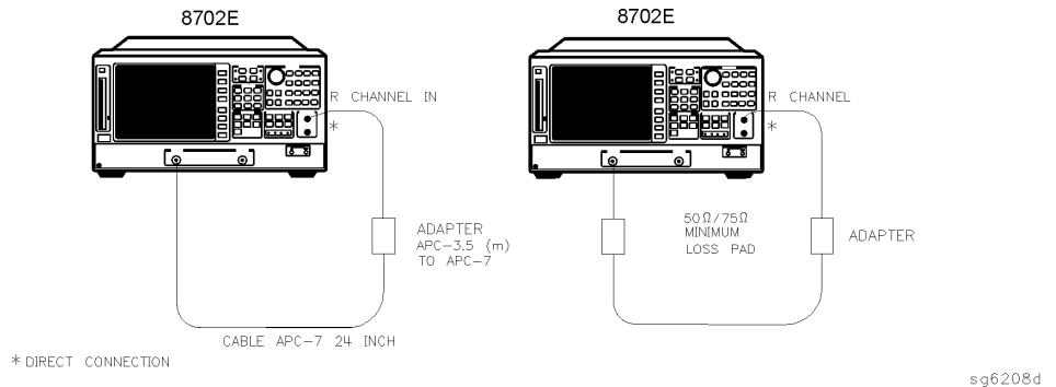
Figure 4-5. Minimum R Channel Level Test Setup
