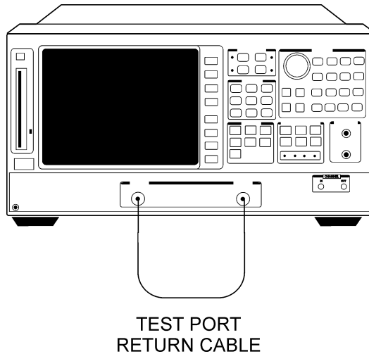
Figure 1-11. Transmission Mode Connections
