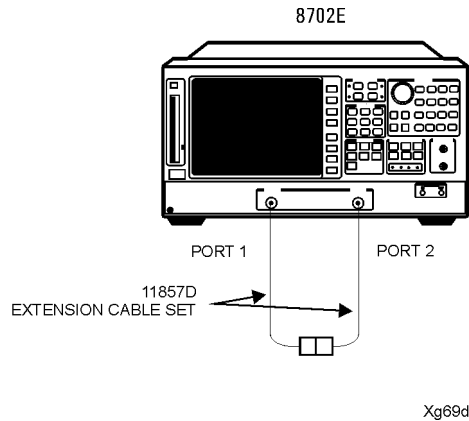
Figure 2-3. Transmission Calibration Setup
