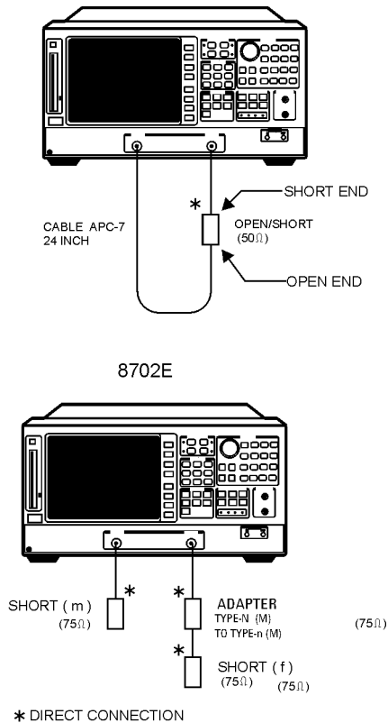
Figure 4-18. Test Port Crosstalk Test Setup
