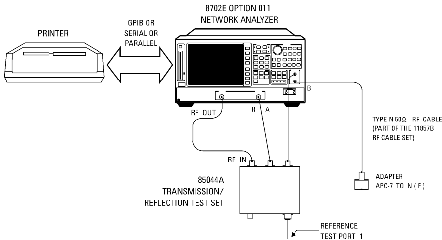
Figure 5-8. System Verification Test Setup
