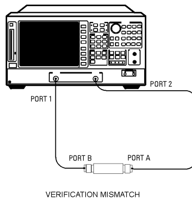
Figure 2-7. Mismatch Device Verification Setup
