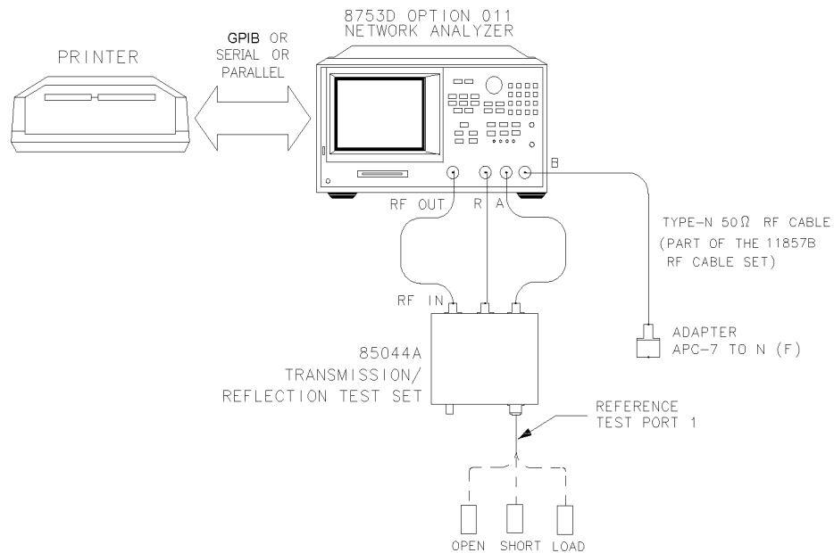
Figure 5-9. Connections for Measurement Calibration Standards
