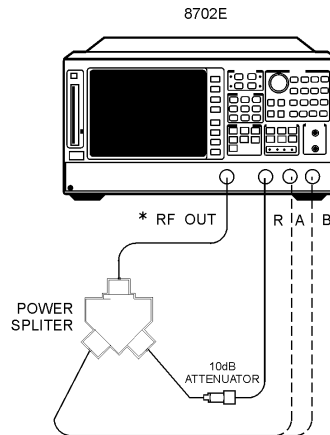
Figure 6-34. Receiver Harmonics Test Setup
