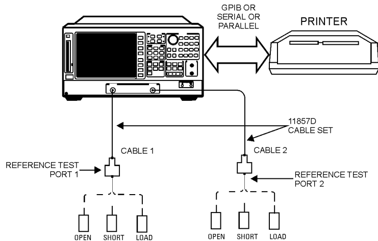
Figure 2-2. Connections for Measurement Calibration Standards
