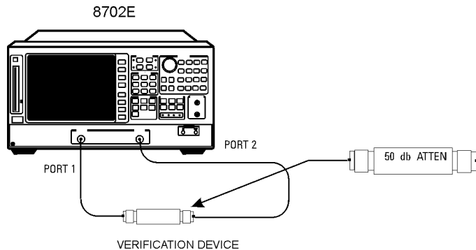
Figure 2-5. Connections for the 50 dB Verification Device
