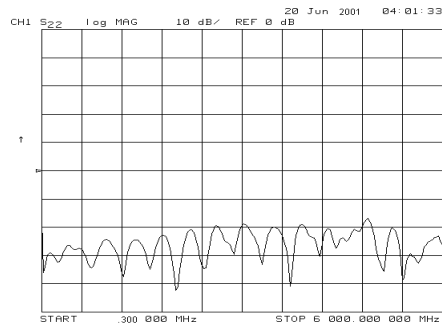
Figure 1-16. Reverse Reflection Mode
