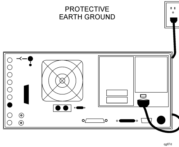
Figure 1-5. Power Cord Connection
