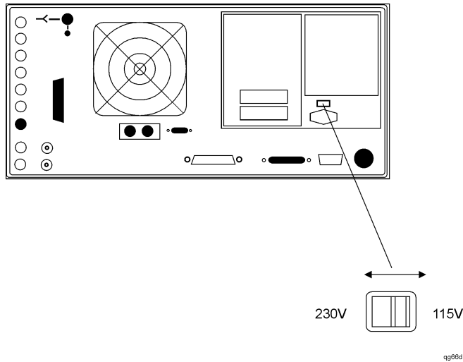
Figure 1-4. Line Voltage Selector
