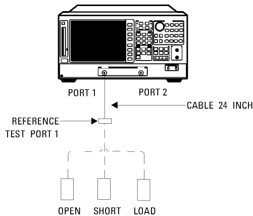
Figure 4-26. S11 1-Port Cal Test Setup
