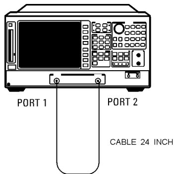
Figure 4-25. System Trace Noise Test Setup
