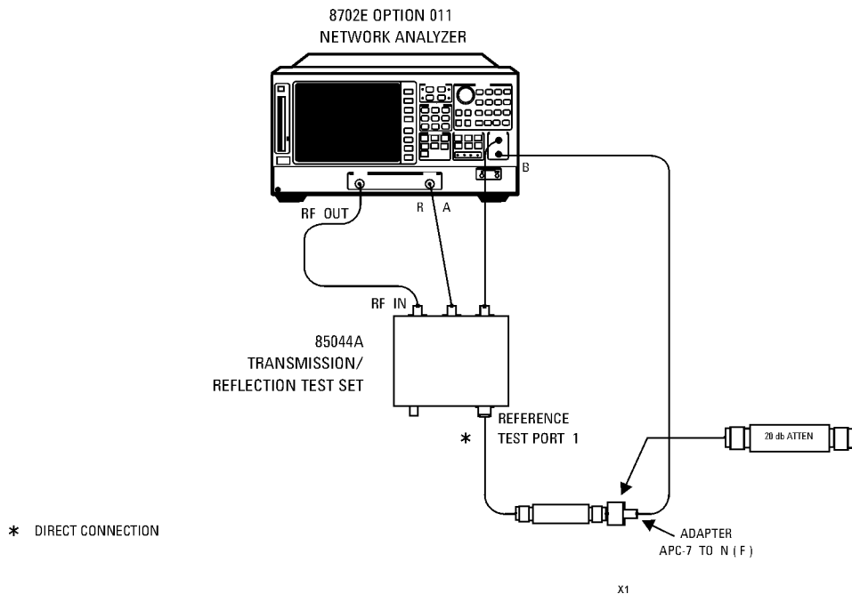
Figure 5-11. Connections for the 20 dB Attenuator
