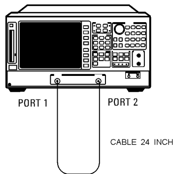
Figure 4-21. Transmission Calibration Test Setup
