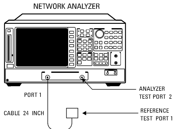
Figure 4-22. Second Full 2-Port Calibration Test Setup
