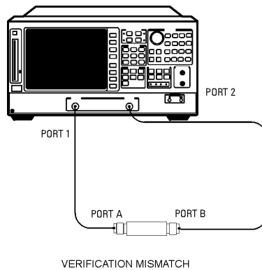
Figure 3-5. Mismatch Device Verification Setup
