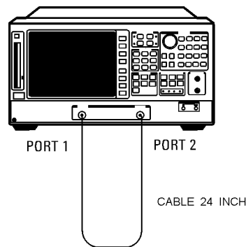
Figure 4-23. Transmission Calibration Test Setup
