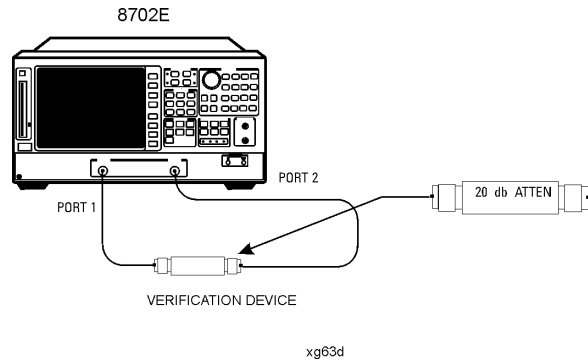
Figure 2-4. Connections for the 20 dB Verification Device
