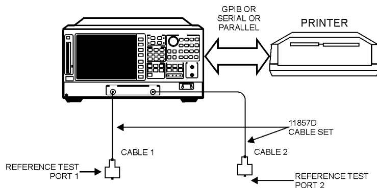
Figure 2-1. System Verification Test Setup
