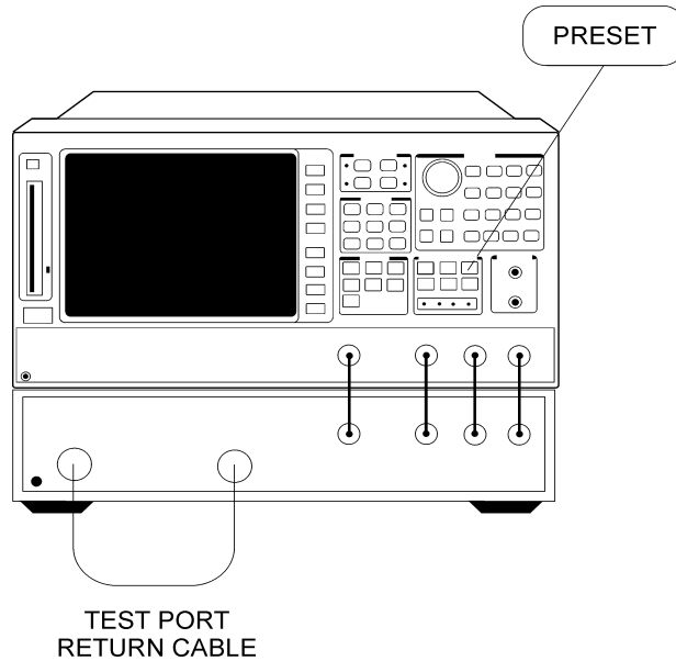
Figure 1-22. Transmission Load Match Connections
