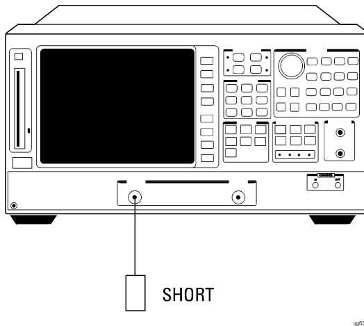
Figure 1-10. Operation Check Connections
