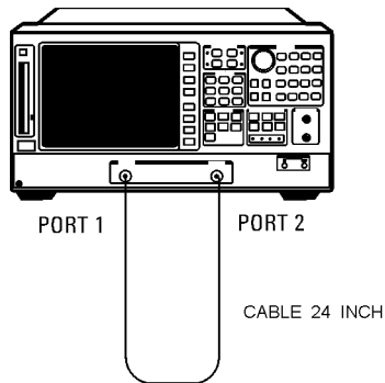
Figure 4-24. System Trace Noise Test Setup
