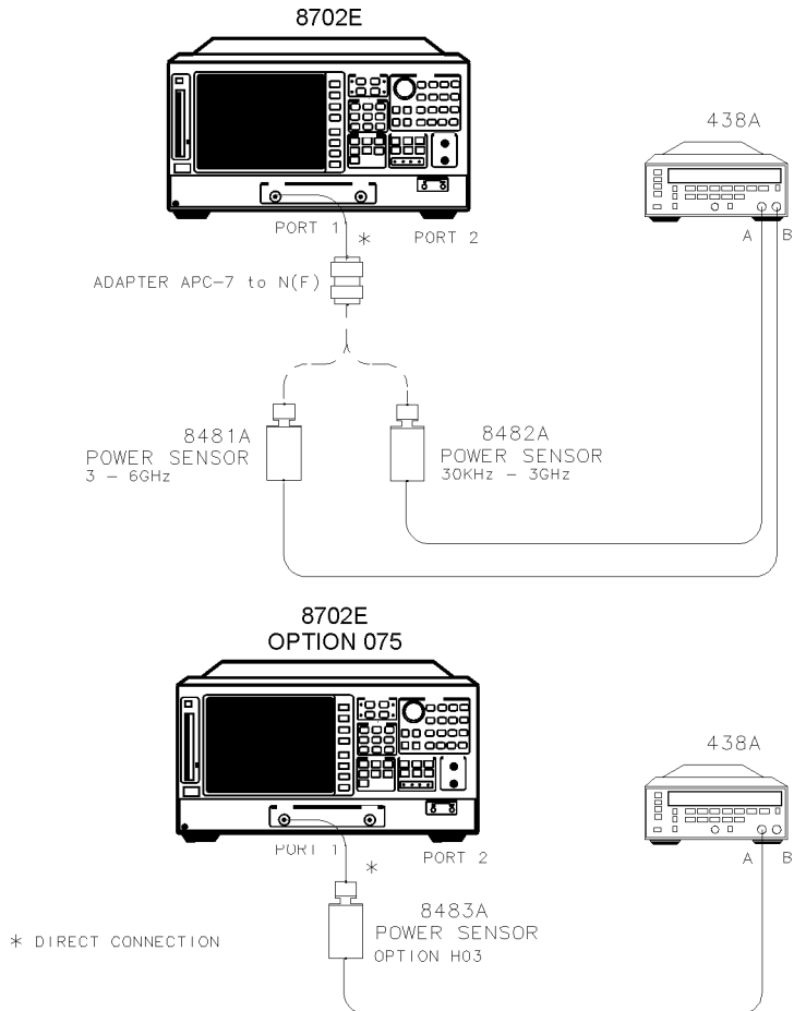
Figure 4-3. Source Output Power Accuracy Test Setup
