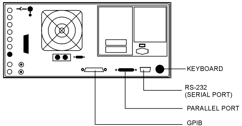
Figure 1-6. Rear Panel Peripheral Connections
