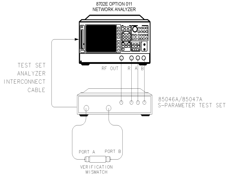
Figure 5-6. Mismatch Device Verification Setup
