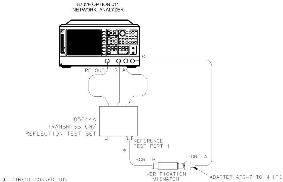
Figure 5-14. Mismatch Device Verification Setup
