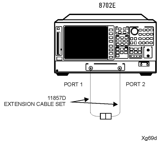
Figure 3-2. Transmission Calibration Setup
