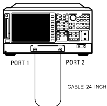
Figure 6-20. Receiver R Input Impedance Test Setup
