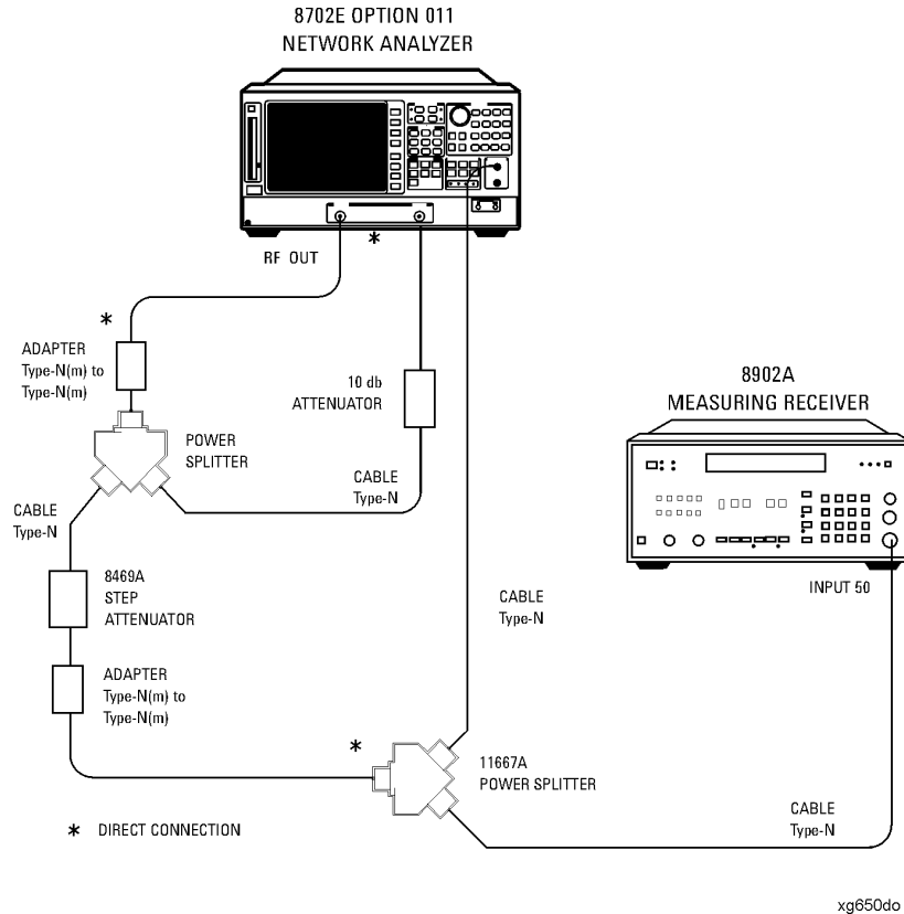
Figure 6-22. Channel A Magnitude Dynamic Accuracy Test Setup
