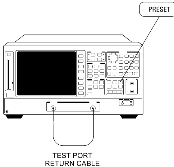
Figure 1-14. Transmission Load Match Connections
