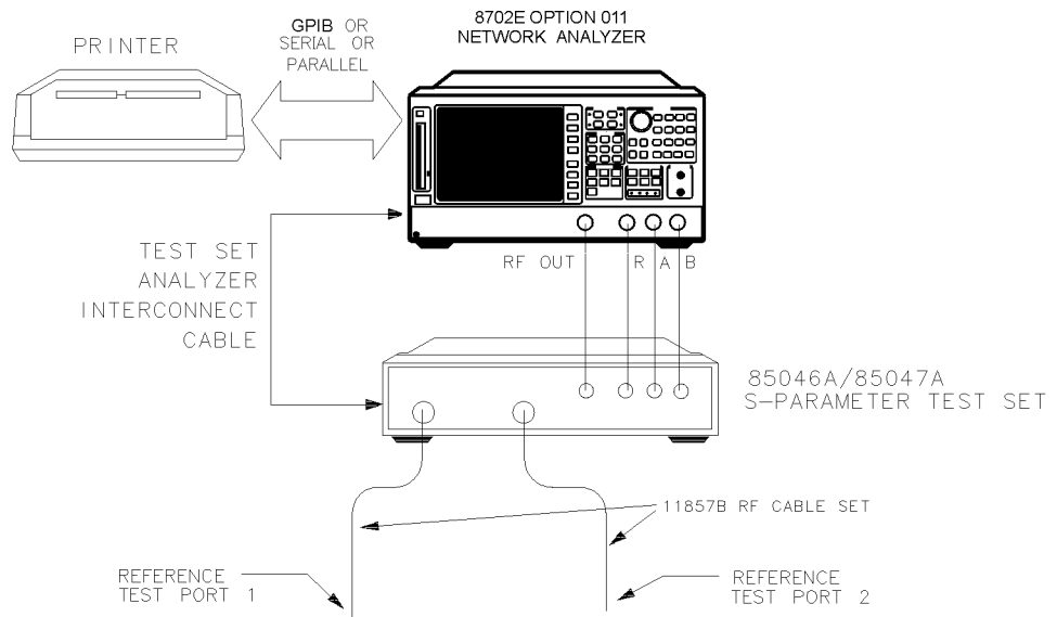
Figure 5-1. System Verification Test Setup
