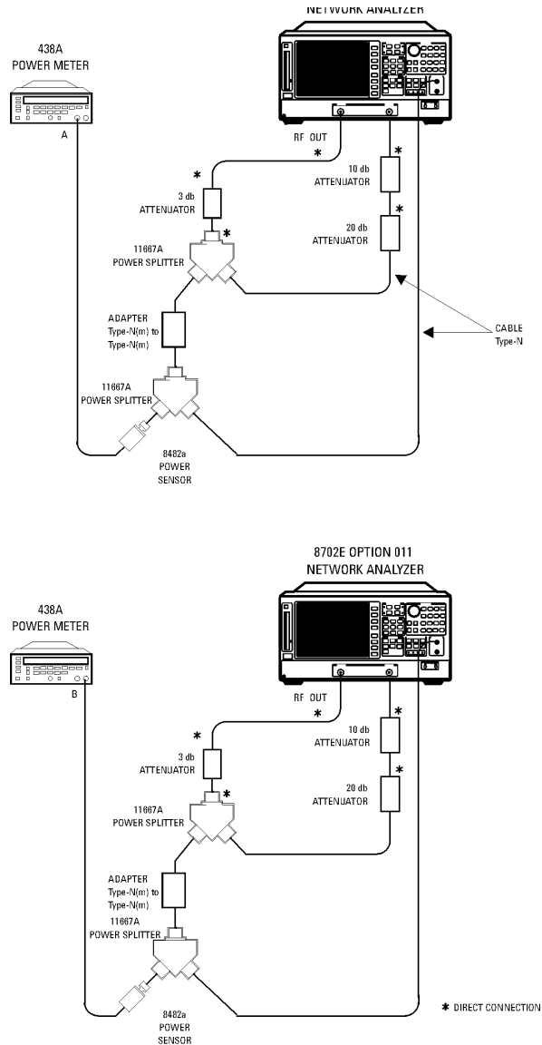
Figure 6-27. Channel B Magnitude Compression Test Setup
