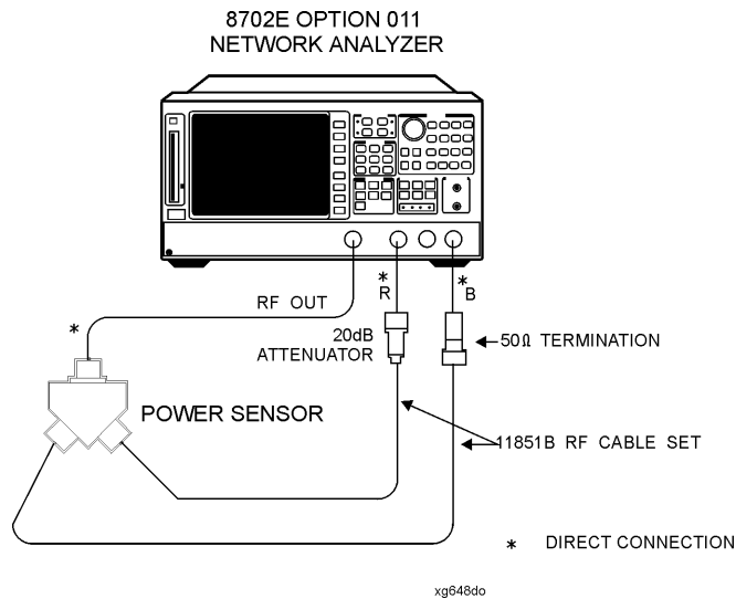
Figure 6-15. A into B Receiver Input Crosstalk Test Setup
