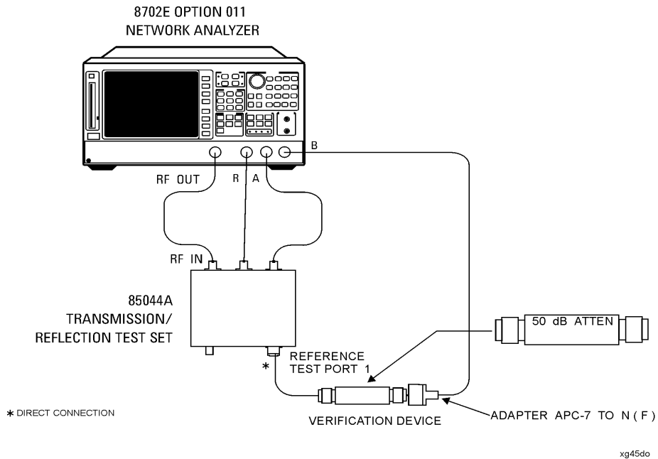
Figure 5-12. Connections for the 50 dB Attenuator
