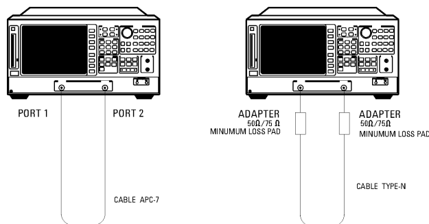
Figure 4-37. Receiver Harmonics Test Setup
