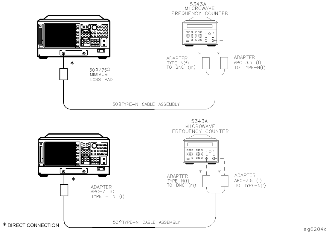
Figure 4-1. Test Port Output Frequency Range and Accuracy Test Setup
