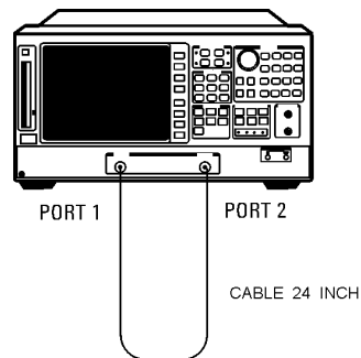
Figure 4-35. Test Port Phase Compression Test Setup
