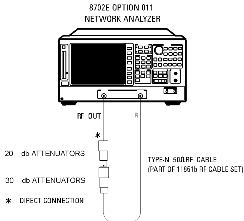
Figure 6-5. Receiver Minimum R Channel Level Test Setup
