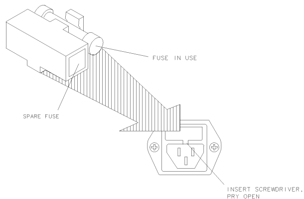
Figure 1-3. Line Fuse Removal and Replacement
