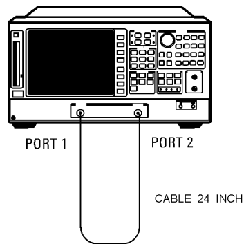
Figure 4-29. Test Port 1 Input Impedance Test Setup
