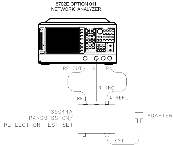
Figure 6-18. Receiver A Input Impedance Test Setup
