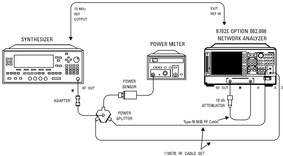
Figure 6-35. Magnitude Frequency Response Test Setup
