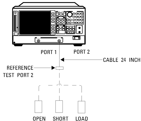
Figure 4-28. S22 1-Port Cal Test Setup
