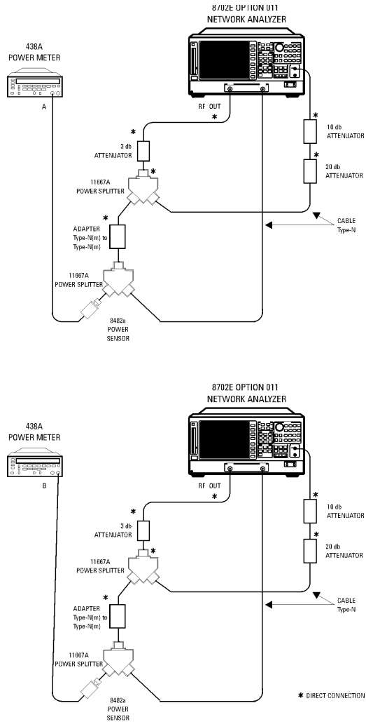
Figure 6-31. Channel R Phase Compression Test Setup
