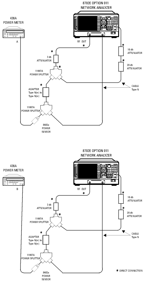
Figure 6-28. Channel R Magnitude Compression Test Setup
