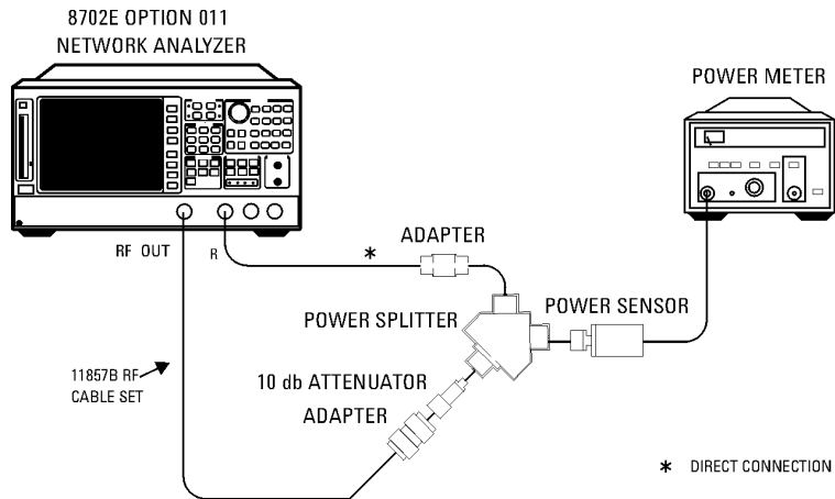
Figure 6-10. Magnitude Frequency Response Test Setup (Receiver Input A)
