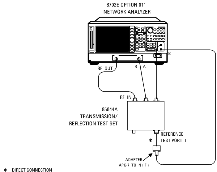
Figure 5-10. Transmission Calibration Setup
