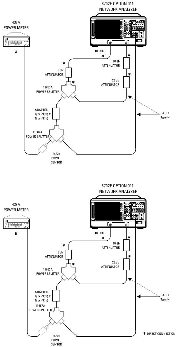
Figure 6-26. Channel A Magnitude Compression Test Setup
