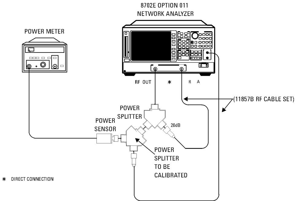
Figure 6-3. Path Loss Calibration Test Setup (#2)
