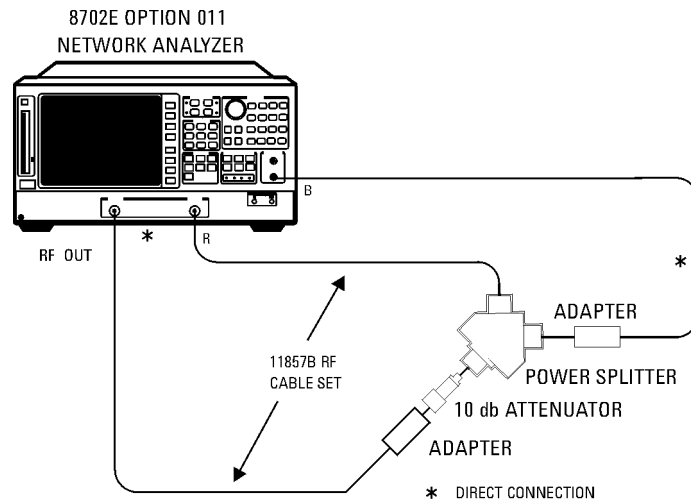
Figure 6-11. Magnitude Frequency Response Test Setup (Receiver Input B)
