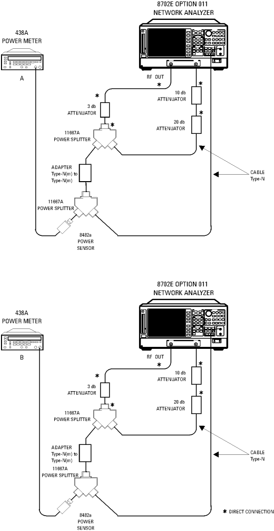
Figure 6-29. Channel A Phase Compression Test Setup
