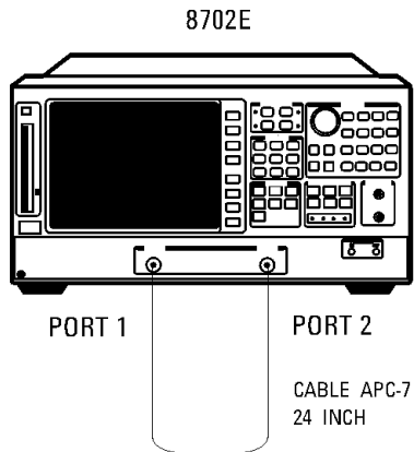
Figure 4-39. Receiver Harmonics Test Setup
