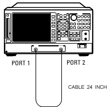
Figure 4-17. Test Port 2 Input Frequency Response Test Setup
