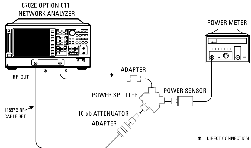
Figure 6-9. Magnitude Frequency Response Test Setup (Receiver Input R)
