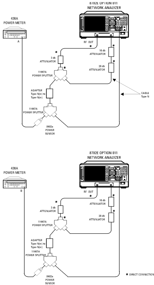
Figure 6-30. Channel B Phase Compression Test Setup
