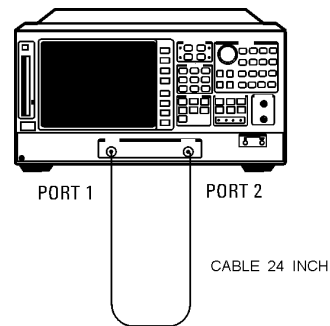
Figure 4-34. Test Port Magnitude Compression Test Setup
