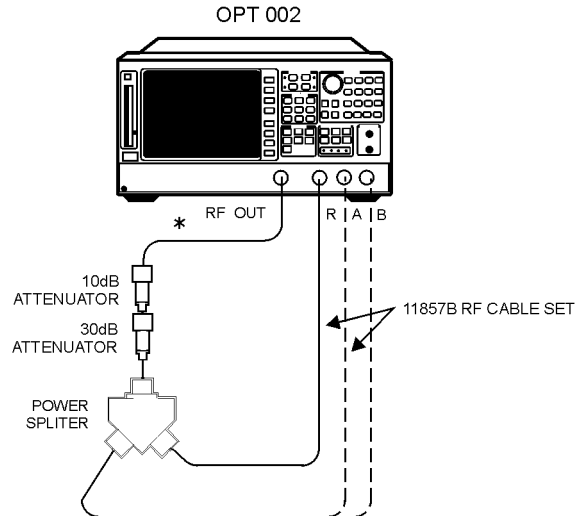
Figure 6-32. Source Harmonics Test Setup
