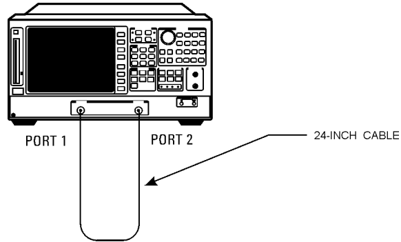
Figure 4-27. Test Port 2 Input Impedance Test Setup
