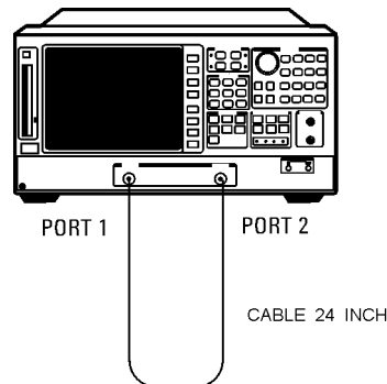
Figure 4-15. Setup for Test Port 1 Input Frequency Response
