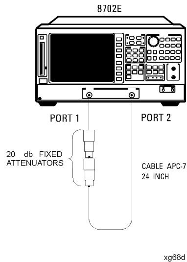
Figure 4-38. Test Port Output Harmonics Test Setup
