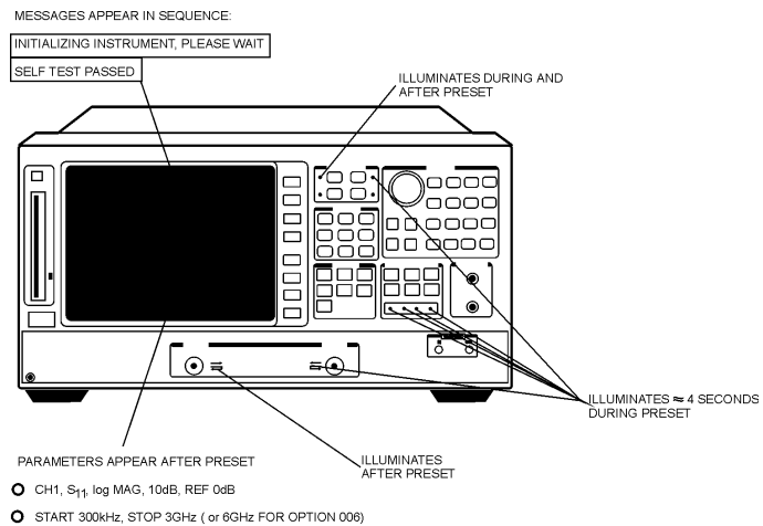
Figure 1-9. Checking the Operation
