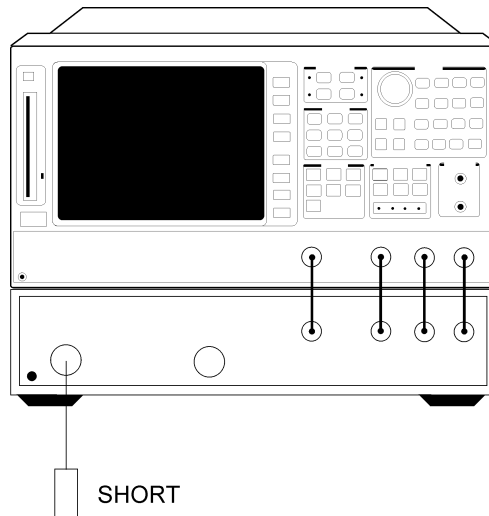
Figure 1-18. Operation Check Connections
