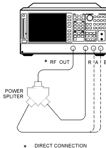
Figure 6-33. Source and Receiver Harmonics Test Setup
